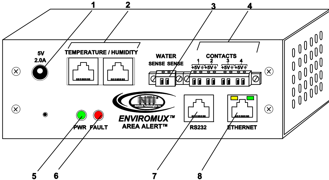
Front View of ENVIROMUX-MINI
