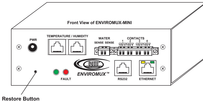
Figure 24- Location of the Restore button
