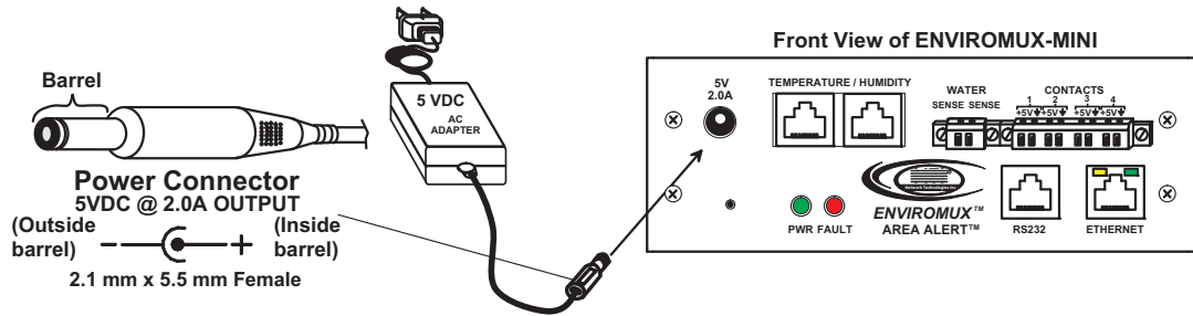
Figure 6- Connect the AC adapter and power-up
