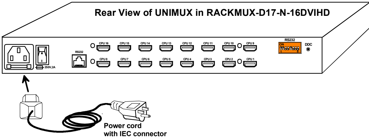
Figure 4- Connect the power cord
