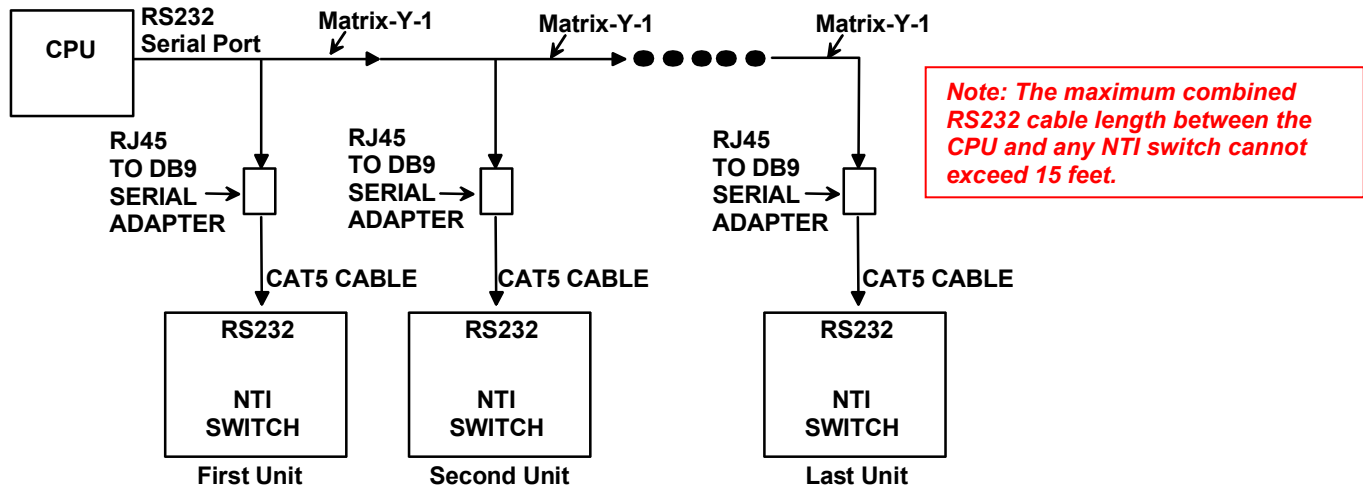
Figure 9- RS232 connection with Matrix-Y-1 cable
