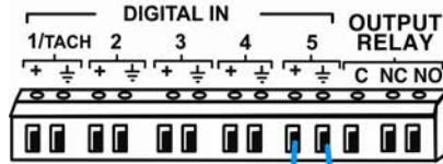
VIEW OF TERMINALS ON E-2D
