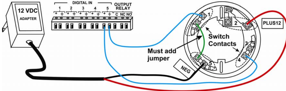
VIEW OF TERMINALS ON E-MINI-LXO
