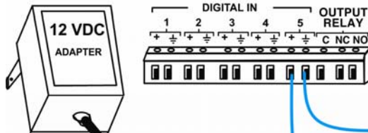
VIEW OF TERMINALS ON E-MINI-LXO
