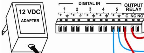
VIEW OF TERMINALS ON E-MINI-LXO
