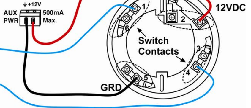
VIEW OF WIRE TERMINALS ON BASE OF E-SDS(-CE)
