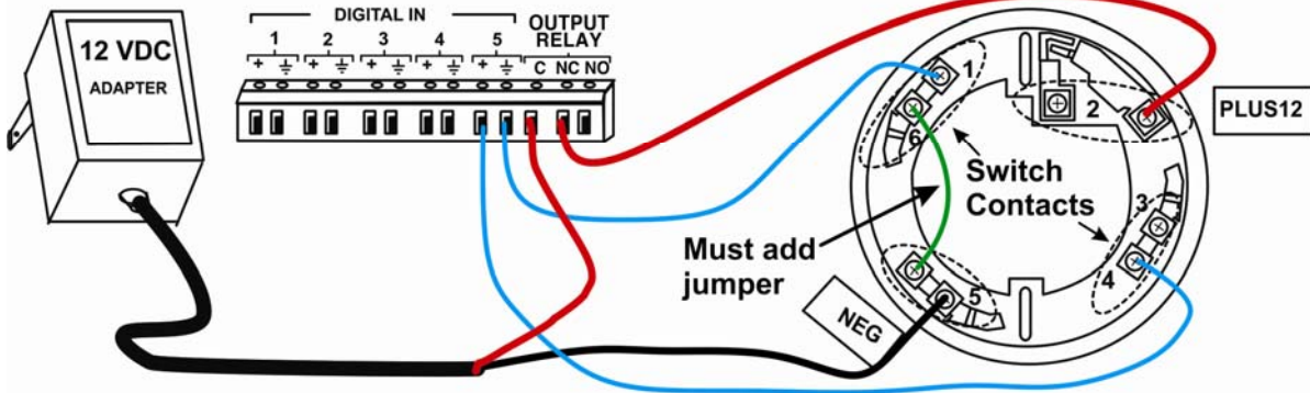
VIEW OF WIRE TERMINALS ON BASE OF E-SDS(-CE)PA
