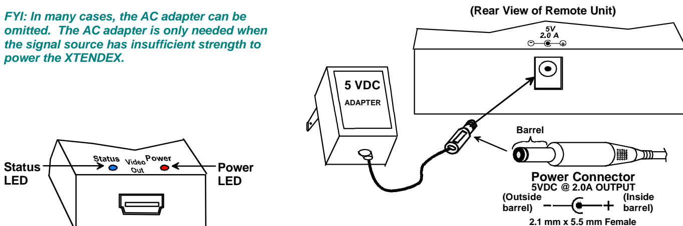
Figure 4- Connect the AC adapter to the Remote Unit
