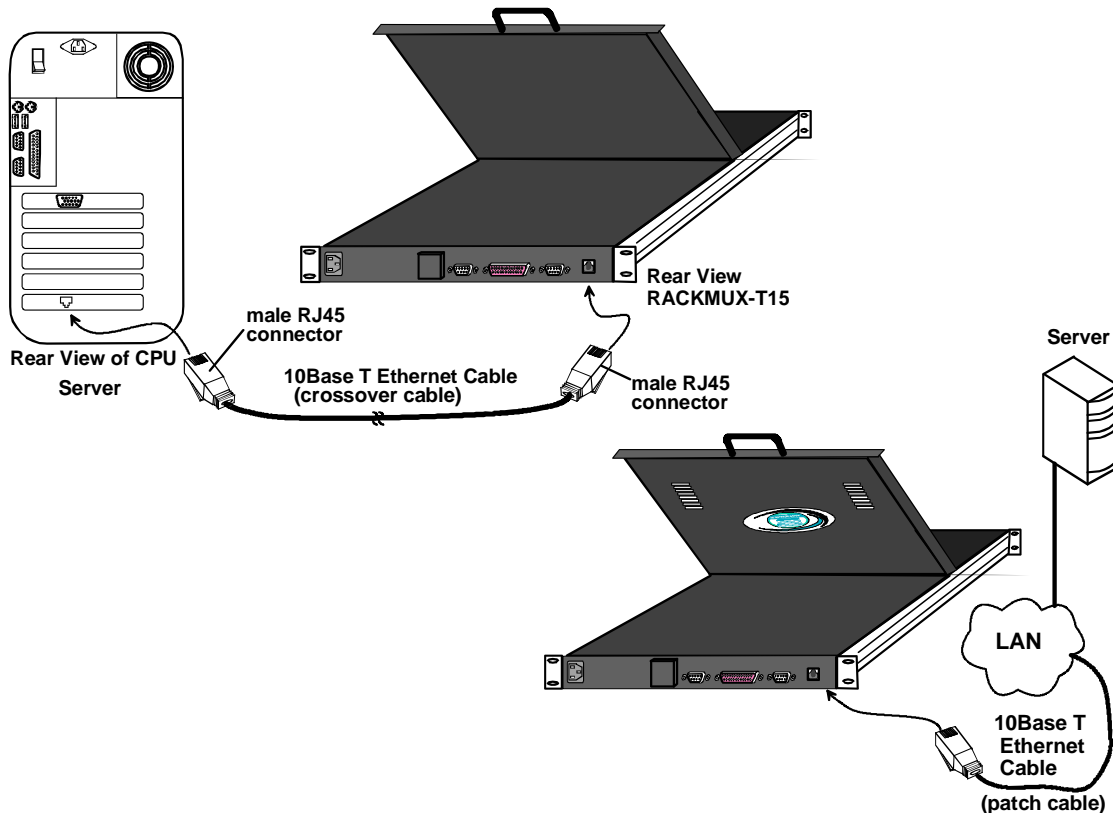
Figure 5- Connect to CPU using Ethernet cable
