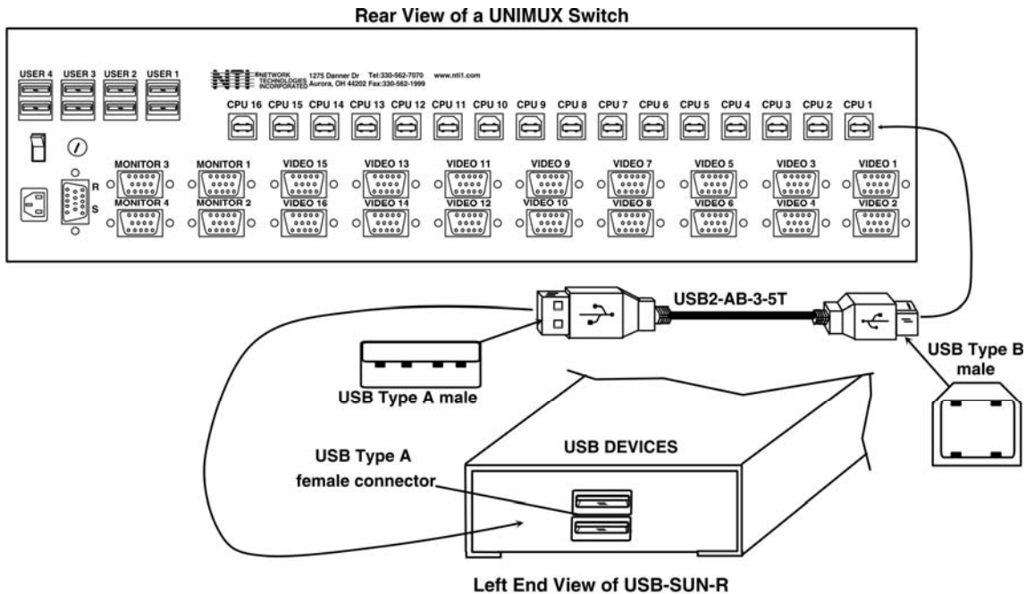
Figure 2- Connect the USB-SUN-R to a UNIMUX switch
