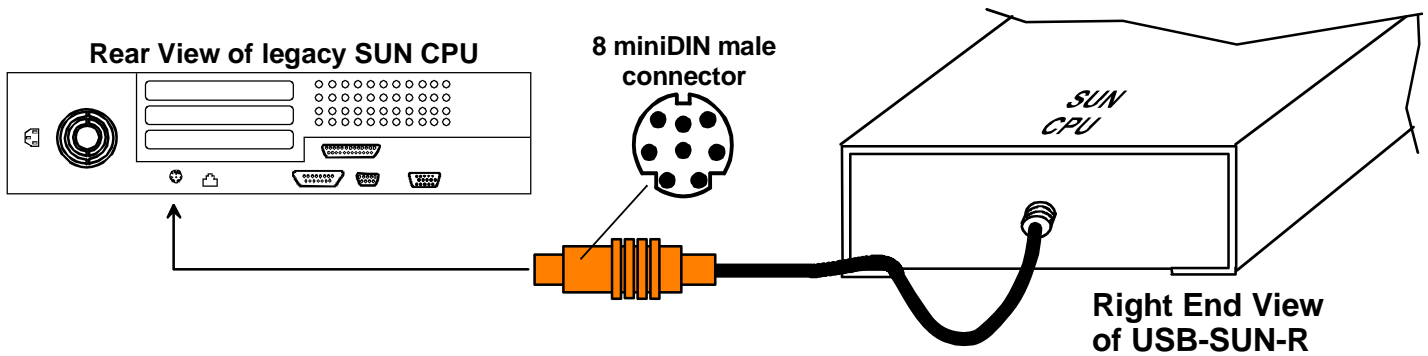
Figure 1- Connect to a legacy SUN CPU
