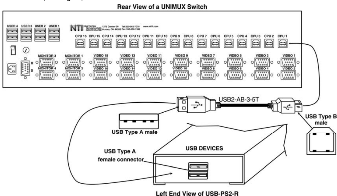
Figure 6- Connect to a PS/2 CPU
