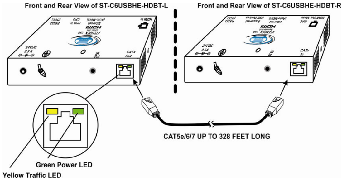
Figure 3- Connect CATx cable
