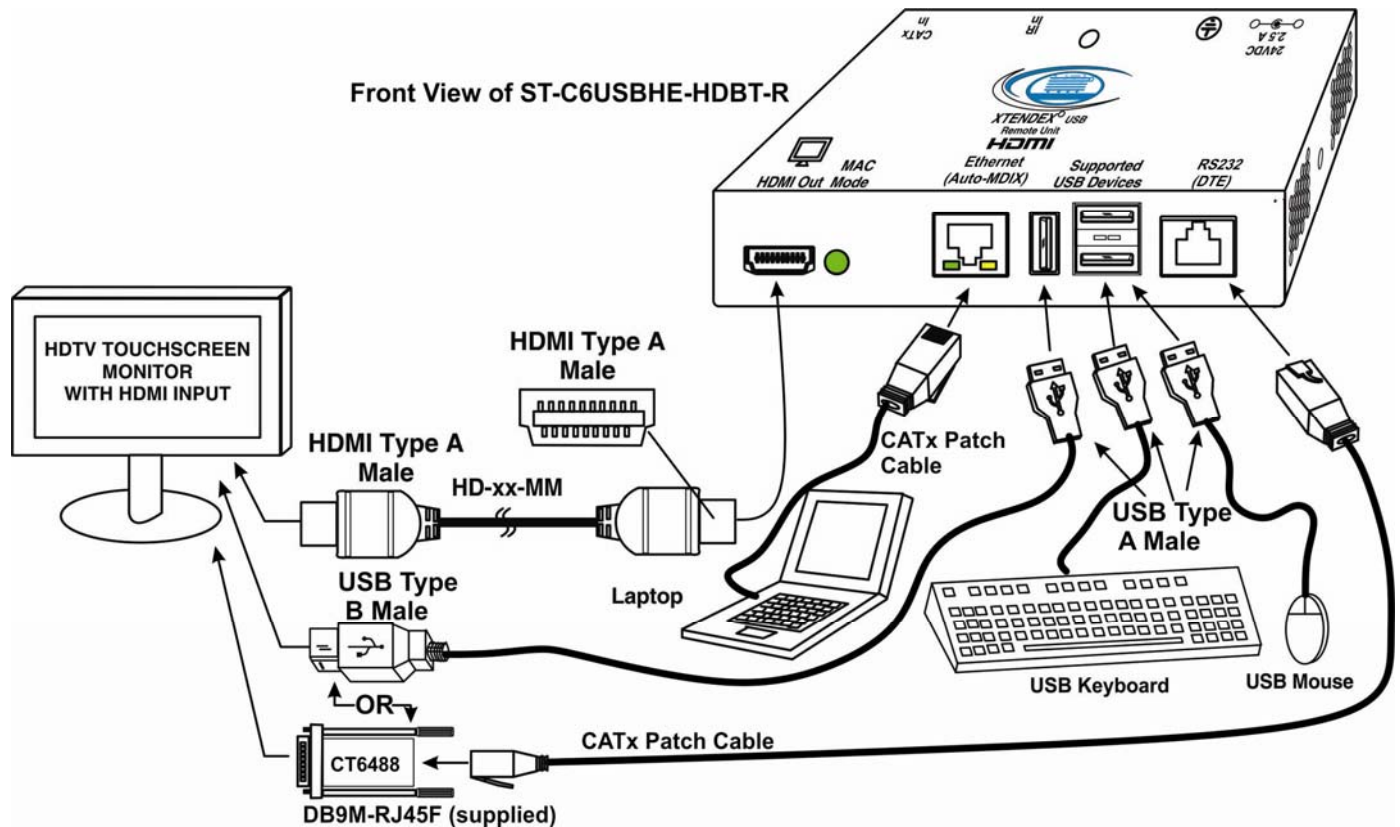
Figure 2- Connect the extended components to the Remote Unit
