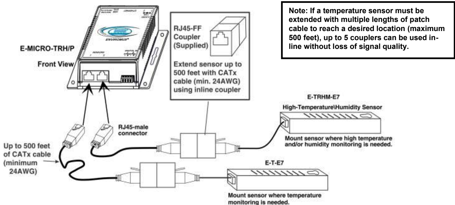
Figure 4- Connect Sensors
