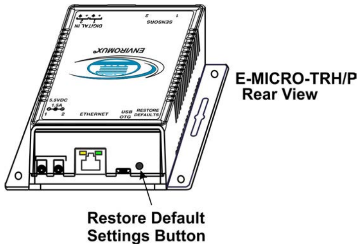
Figure 61- Location of Restore Defaults button
