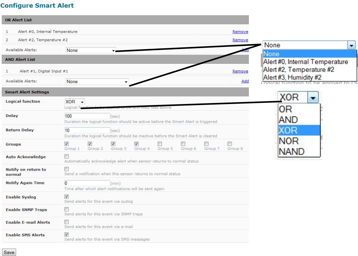
Figure 24- Sensor to be used for a predefined event
