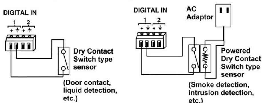
Figure 5- Terminal block for dry-contact sensors
