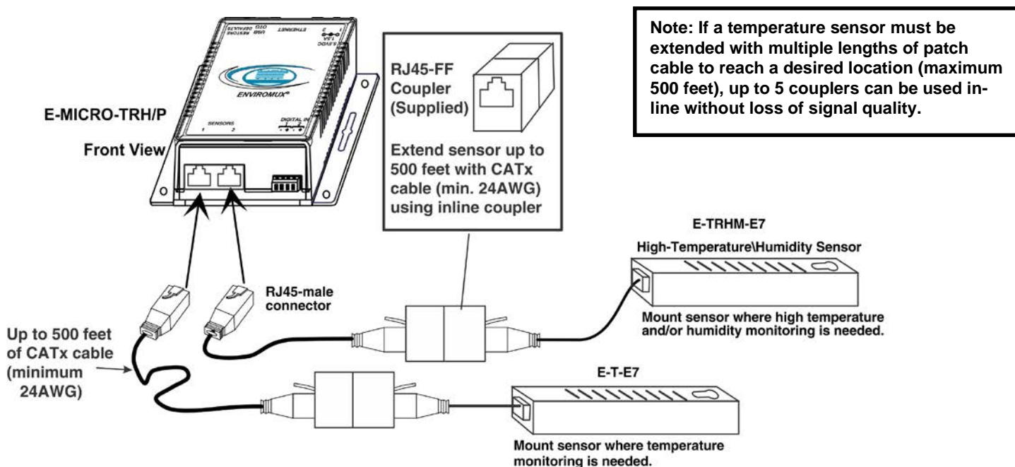
Figure 4- Connect Sensors
